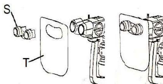
Fig. 11a Mounting breath shield
