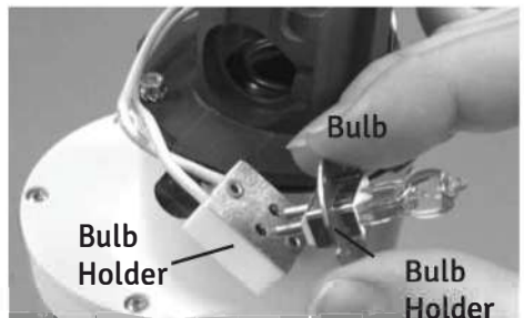
Figure 22b New Bulb
