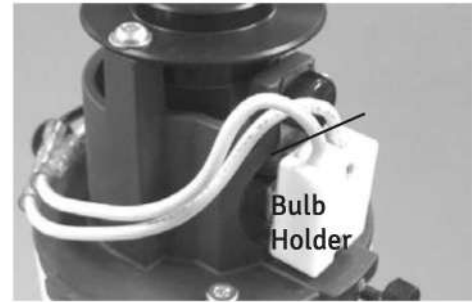
Figure 21 Securing Screw
